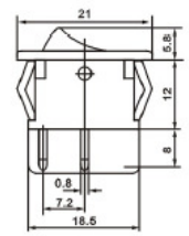
KCD1-201-6 ON-OFF KCD1-201N-6 ON-OFF KCD1-202-6 ON-OFF KCD1-202N-6 ON-ON KCD1-203-6 ON-OFF-ON
