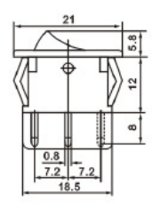
KCD1-201-6 ON-OFF KCD1-201N-6 ON-OFF KCD1-202-6 ON-OFF KCD1-202N-6 ON-ON KCD1-203-6 ON-OFF-ON
