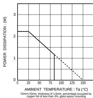
Fig.10 Power dissipation
