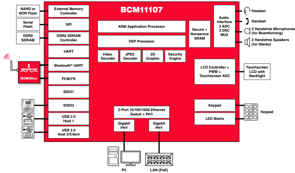
BCM11107 Block Diagram
