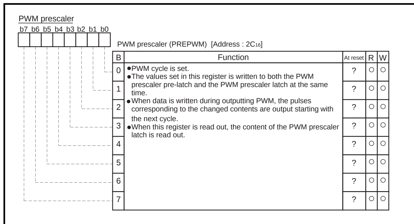
Fig. 2.4.3 Structure of PWM prescaler
