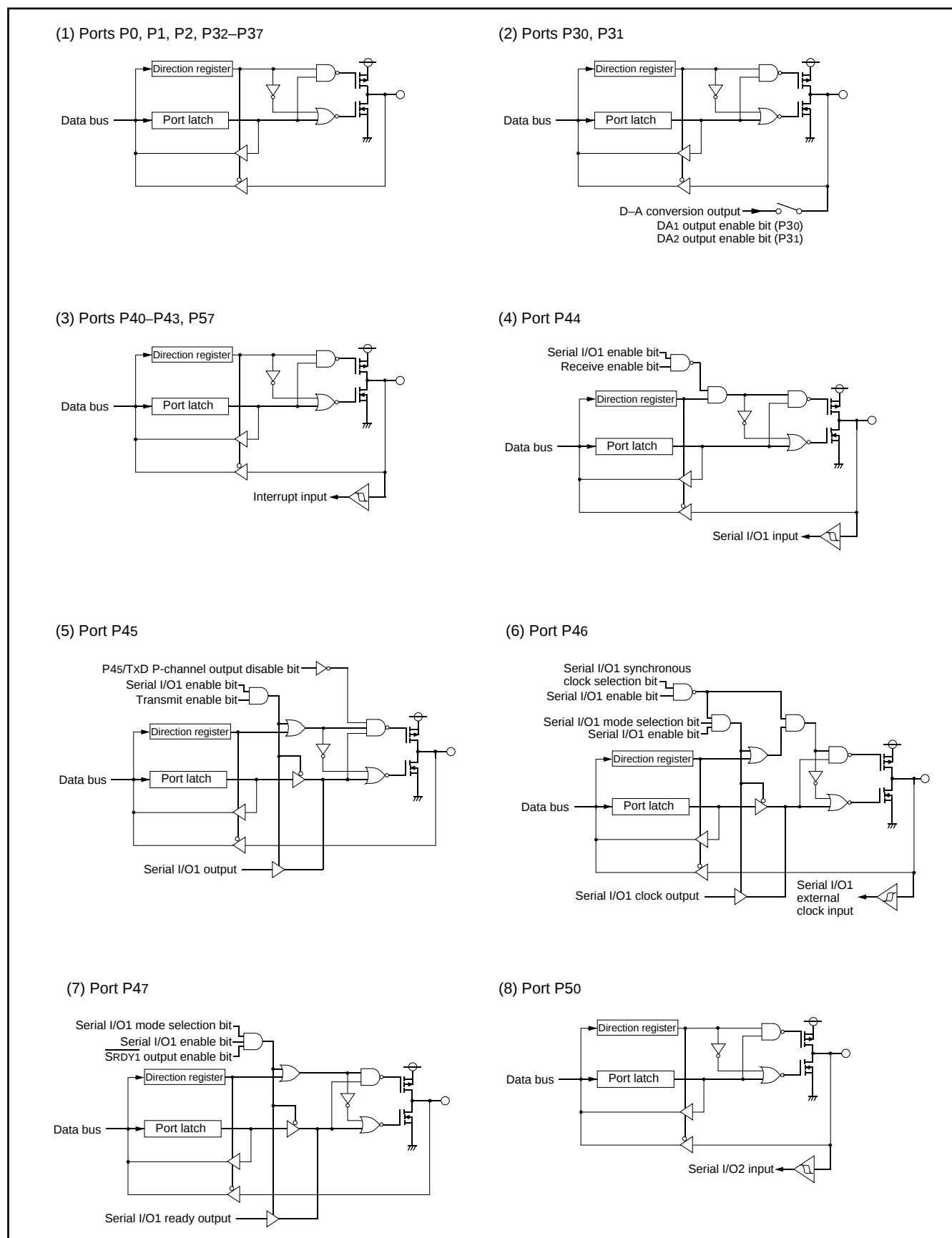
Fig. 12 Port block diagram (single-chip mode) (1)
