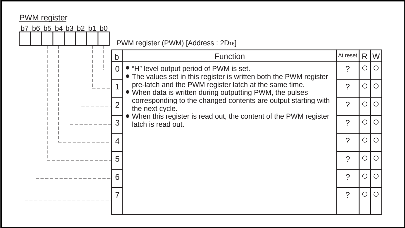
Fig. 2.4.4 Structure of PWM register
