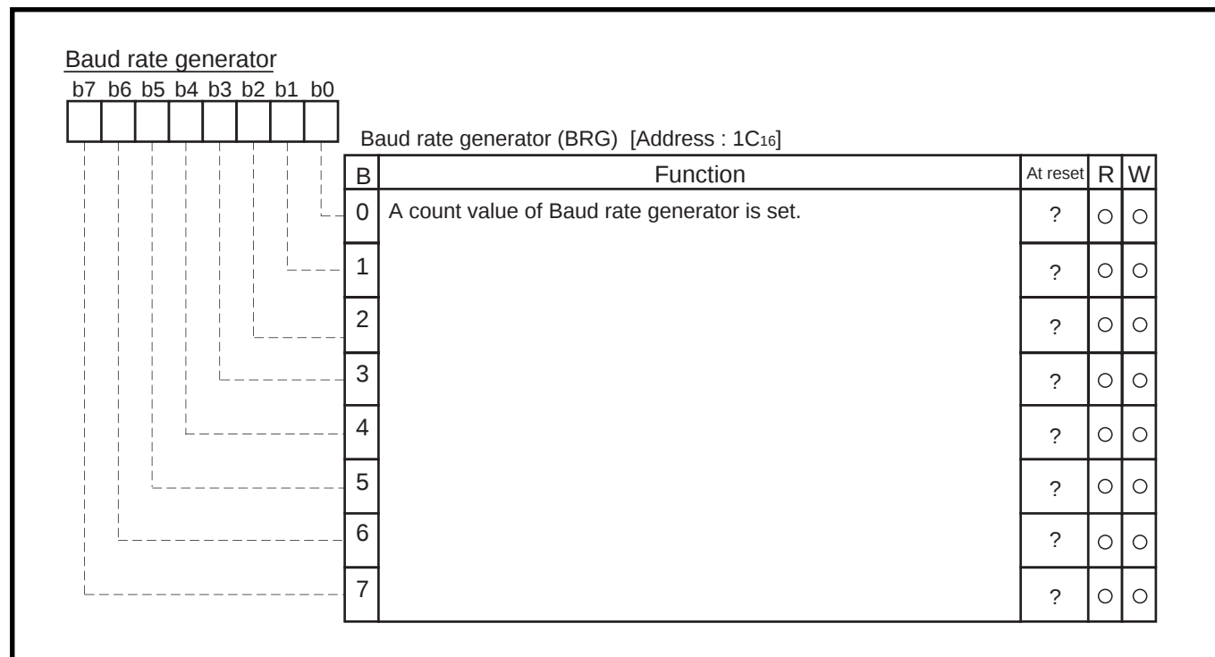
Fig. 2.3.6 Structure of Baud rate generator
