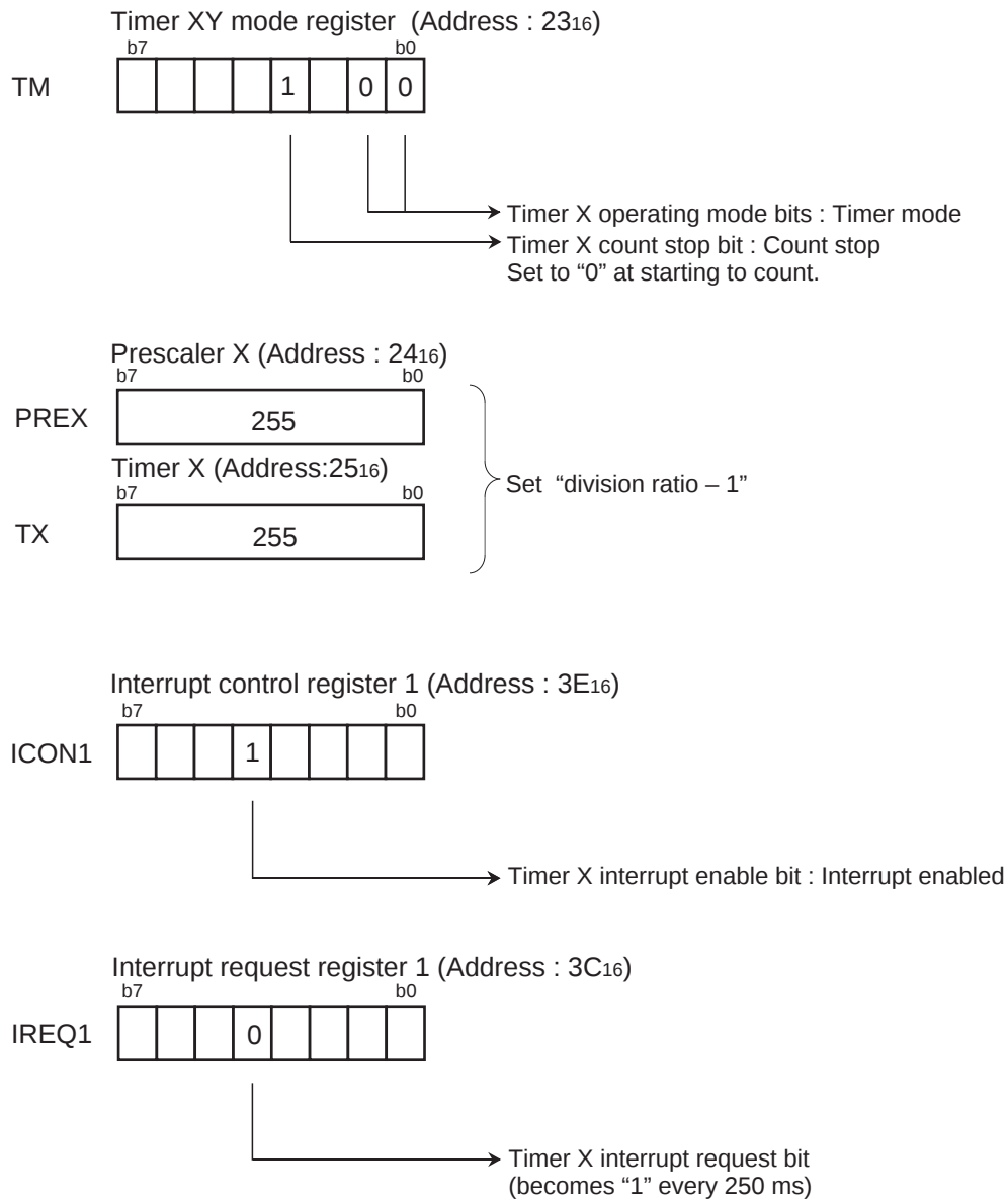
Fig. 2.2.11 Setting of related registers [Clock function]
