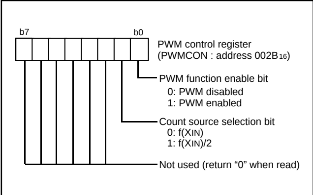
Fig. 28 Structure of PWM control register
