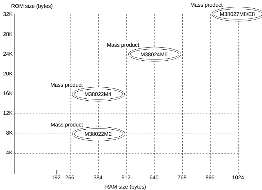
Fig. 5 Memory expansion plan
