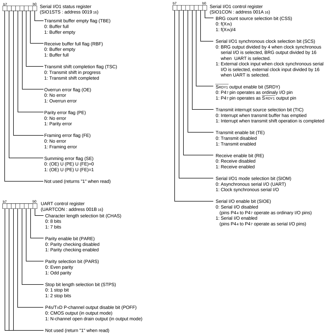
Fig. 22 Structure of serial I/O control registers
