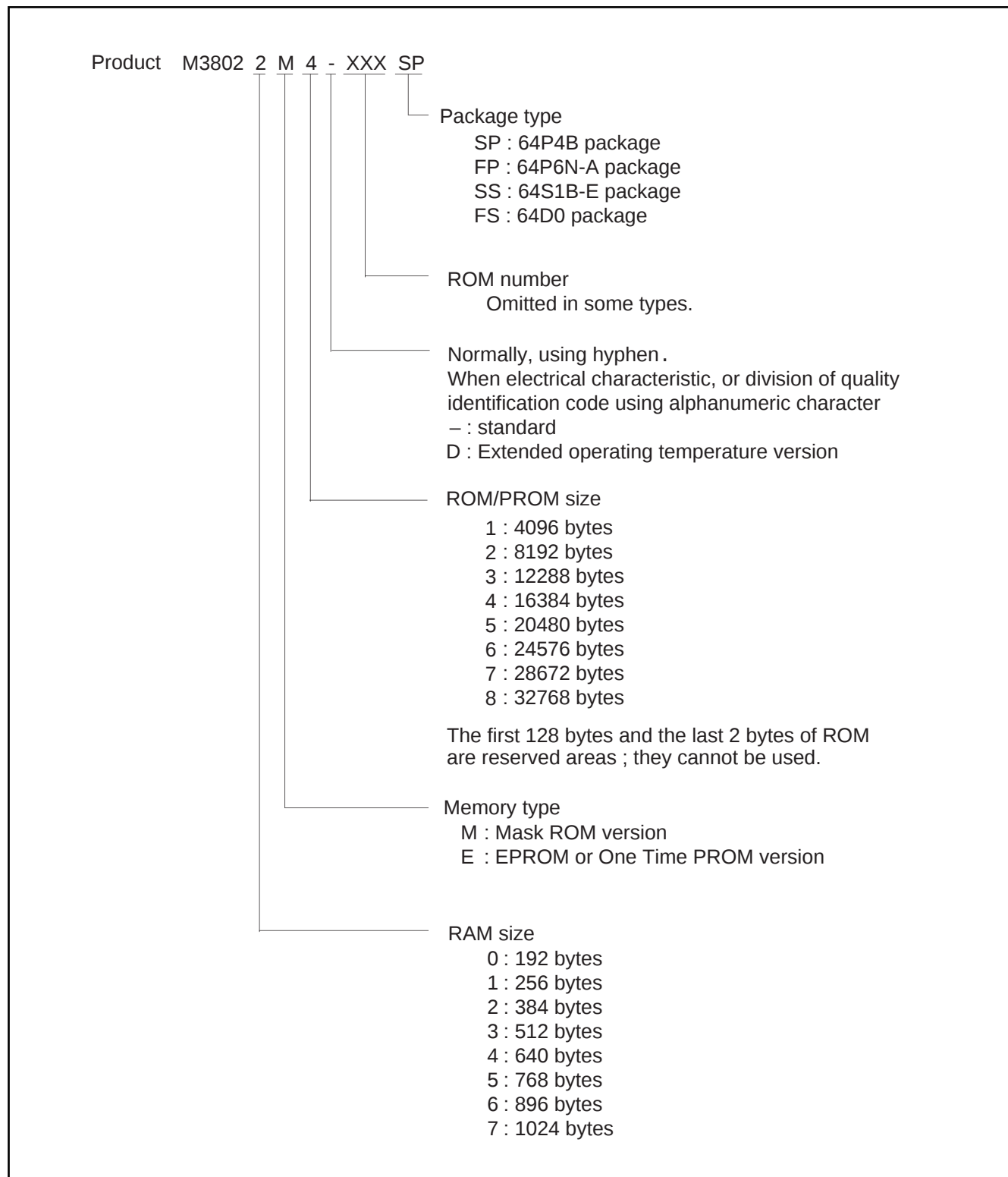
Fig.4 Part numbering
