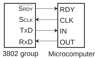
(3) Using the \overline{\text{SRDY}} signal output function (Selecting an external clock)
