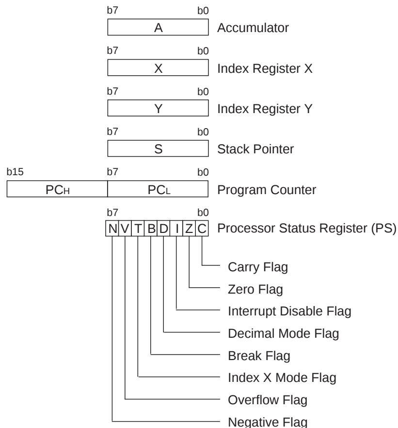
Fig. 7. 740 Family CPU register structure
