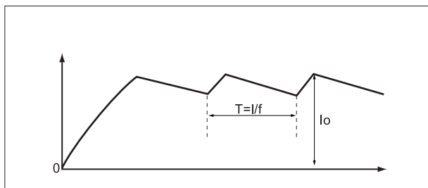
Fig.1 Constant current wave form (Motor current)
