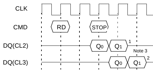
4) Read Burst Stop (BL=4)
