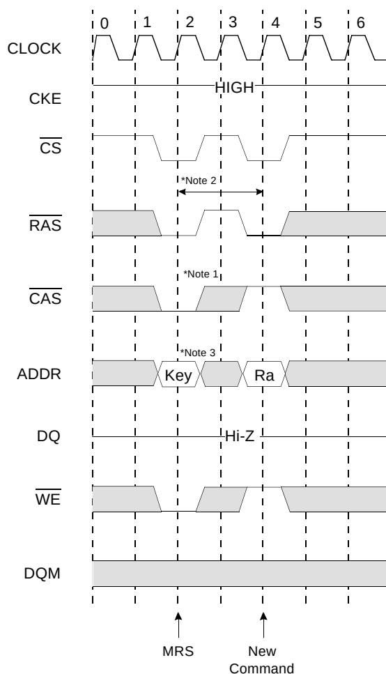
Mode Register Set Cycle
