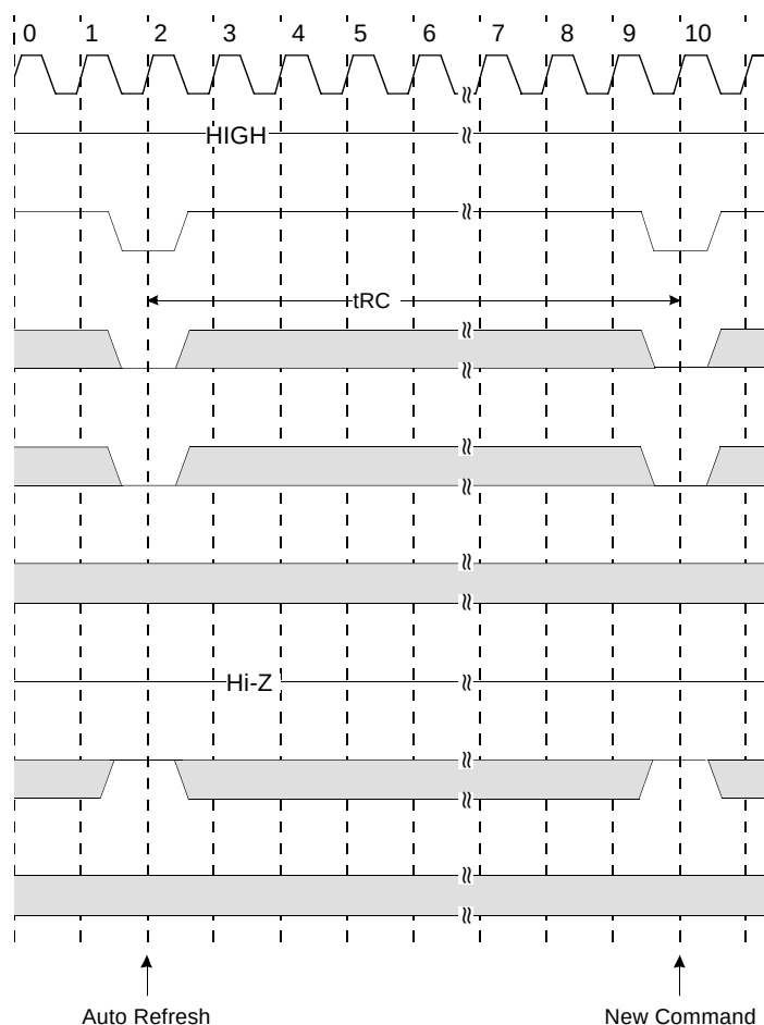
Auto Refresh Cycle
