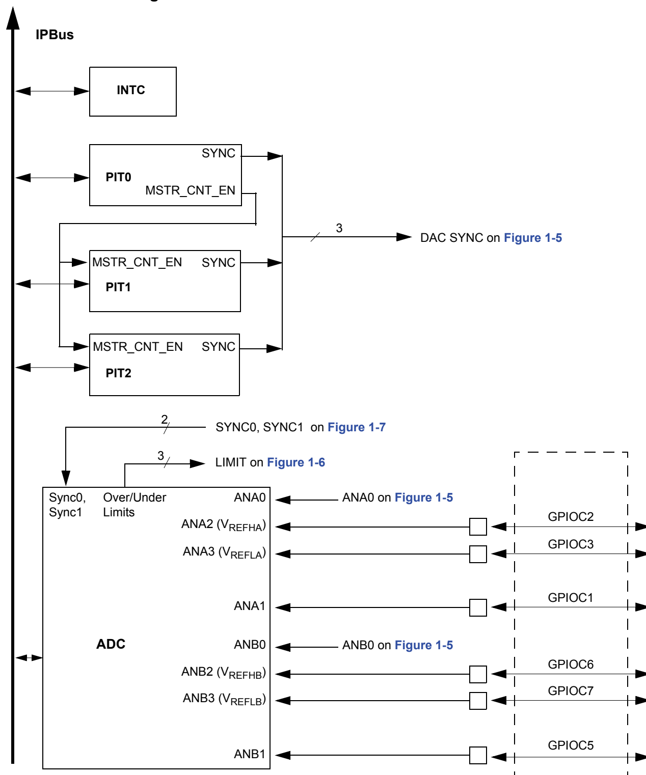
Figure 1-3 56F8025 I/O Pin-Out Muxing (Part 1/5)
