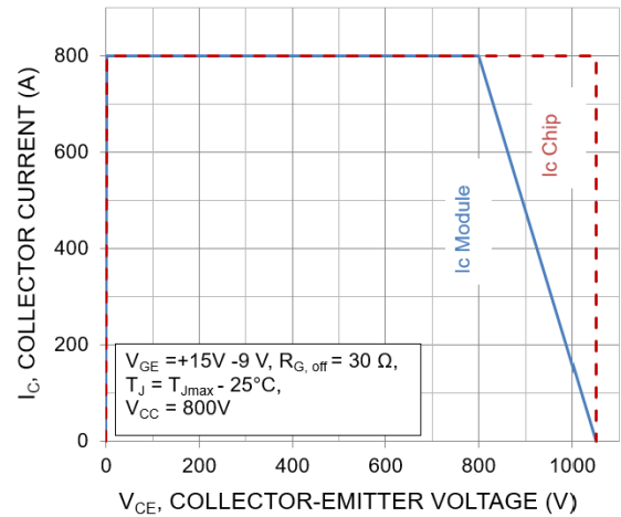
Figure 7. RBSOA (T1–T4)
