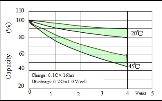
Storage & self discharge Curves of 3000mAh SC Ni-MH Battery
