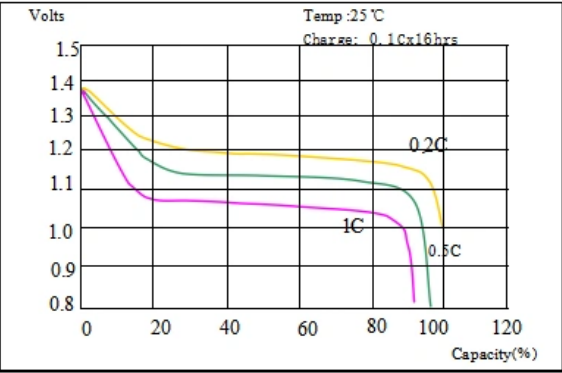
Discharging Curves of 3000mAh SC Ni-MH Battery-0.2C/0.5C/1C
