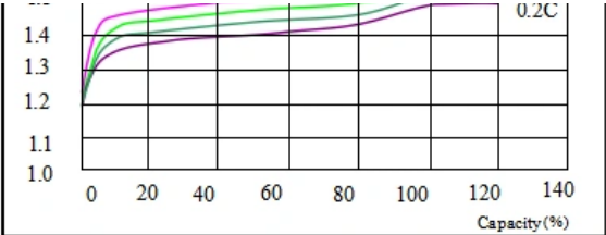
Charging Curves of 3000mAh SC Ni-MH Battery-0.1C/0.2C/0.5C/1.0C
