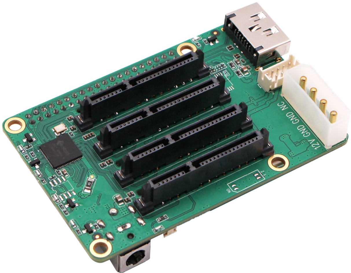
Figure 1: Radxa Penta SATA HAT
