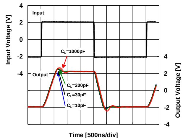
Pulse Response
