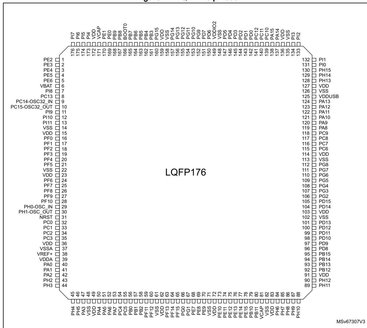
Figure 14. LQFP176 pinout
