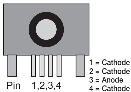
FIGURE 8. PINOUT
