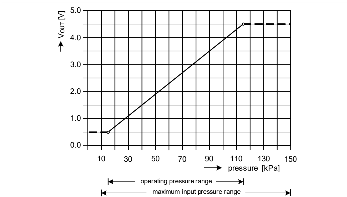
Figure 3 Transfer function
