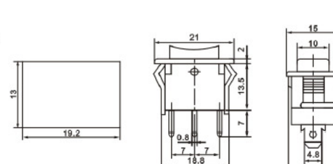
KCD1-103-2 ON-OFF-ON KCD1-123-2 (ON)-OFF-(ON) (双复位)
