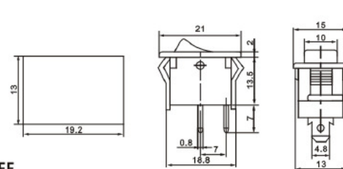
KCD1-101-2 ON-OFF KCD1-111-2 (ON)-OFF (单复位) KCD1-102-2 ON-ON
