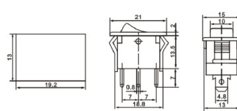
KCD1-101-2 ON-OFF KCD1-111-2 (ON)-OFF (单复位) KCD1-102-2 ON-ON
